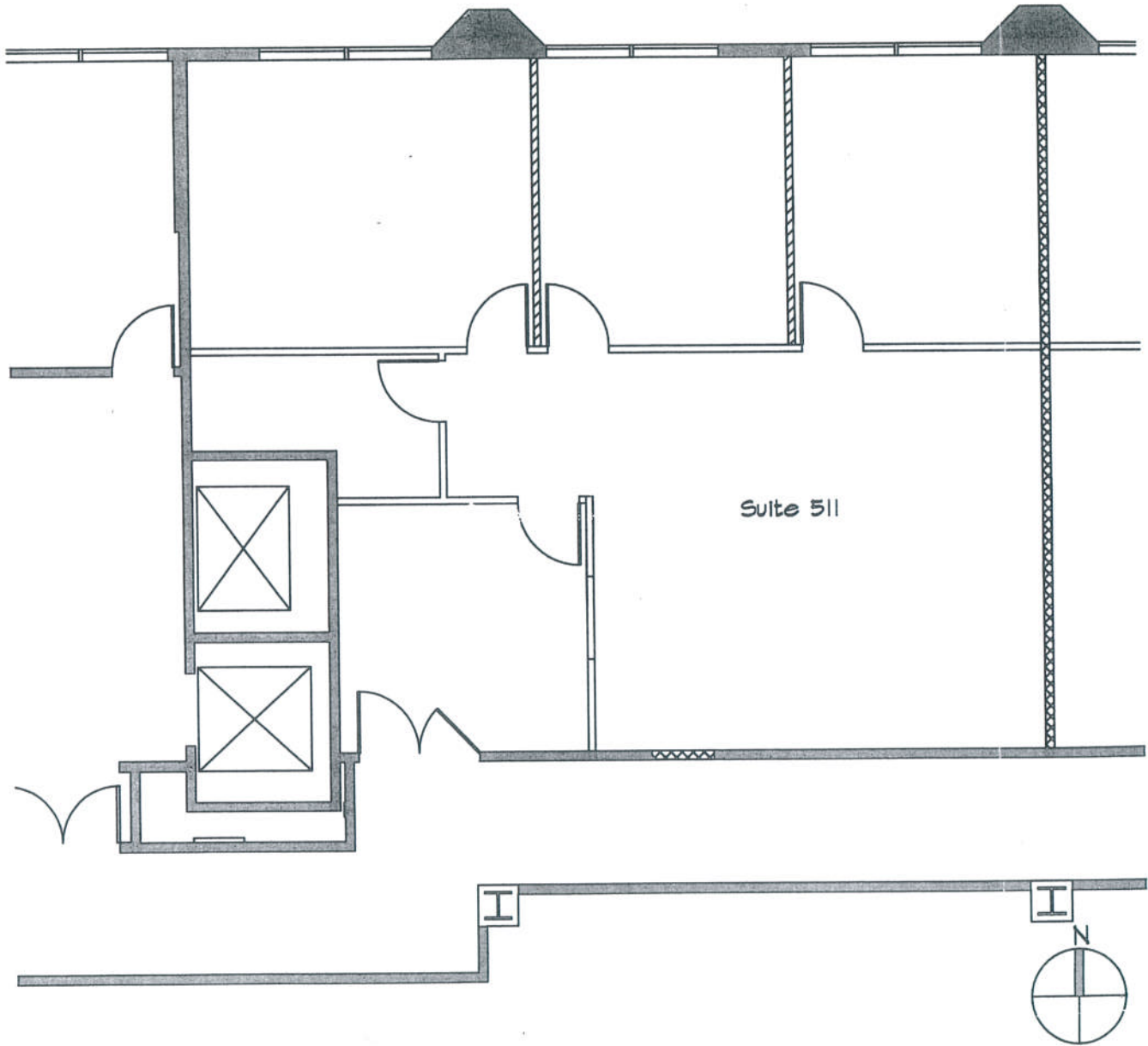
FLOOR PLAN 1/8"=1'-0"
